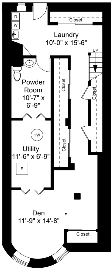
Lower Level Plan Ceiling Height = 6'-4"
