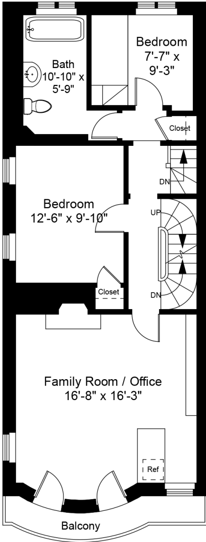
Second Floor Plan Ceiling Height = 9'-1"
